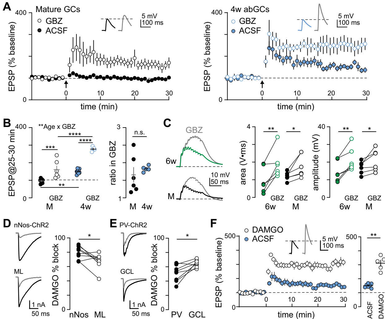
Figure 3. GABA A -mediated inhibition suppresses LTP. A , LTP in perforated patch recordings from mature GCs ( n = 6 ; left) and 4w abGCs ( n = 5 ; right) in GBZ (open symbols), with comparison to results in ACSF (from Fig. 2A, solid symbols). Insets show EPSPs before and after TBS in GBZ. B , Left, Summary data from 25 to 30 min post-TBS. Two-way ANOVA main effect of cell age p < 0.0001 ; main effect of GBZ p < 0.0001 ; interaction effect F_{(1,24)} = 10 , p = 0.005 ; Tukey's post hoc 4w ACSF versus GBZ p < 0.0001 , 4w ACSF versus M ACSF p = 0.001 , 4w GBZ versus M GBZ p < 0.0001 , M ACSF versus GBZ p = 0.0004 . Right, The ratio of LTP in GBZ versus ACSF; unpaired Welch's t test; t_{(5,3)} = 0.78 , p = 0.5 . C , Example depolarizations in 6w or M GCs during TBS using whole-cell recordings ( n = 6 each). GBZ increases the area ( p = 0.0007 ) regardless of cell age ( p = 0.7 ). There was no significant interaction effect between cell age and GBZ (two-way RM ANOVA; F_{(1,10)} = 1.2 , p = 0.3 ; Bonferroni's multiple comparisons 6w p = 0.004 , M p = 0.048 ). GBZ also increases the peak amplitude of depolarization. Two-way RM ANOVA, F_{(1,10)} = 1.7 , p = 0.2 ; main effect of cell age p = 0.8 ; main effect of GBZ p = 0.0003 ; Bonferroni's multiple comparisons 6w p = 0.002 , M p = 0.04 . D , IPSCs in mature GCs evoked by alternating optogenetic stimulation of nNos-ChR2 (top, 1 ms) and electrical stimulation in the ML (bottom) were reduced by DAMGO (gray). Paired t test; t_{(7)} = 2.61 , p = 0.03 ( n = 8 ). E , IPSCs evoked by alternating optogenetic stimulation of PV-ChR2 and electrical stimulation in the GCL (bottom) were suppressed by DAMGO. Paired t test; t_{(7)} = 3.39 , p = 0.01 ( n = 8 ). F , DAMGO enhanced LTP in perforated patch recordings from 4w abGCs ( 312 \pm 22\% ; n = 5 ; perforated patch recordings) compared with ACSF (from Fig. 2A; Welch's t test; t_{(4,5)} = 7.0 , p = 0.001 ).
