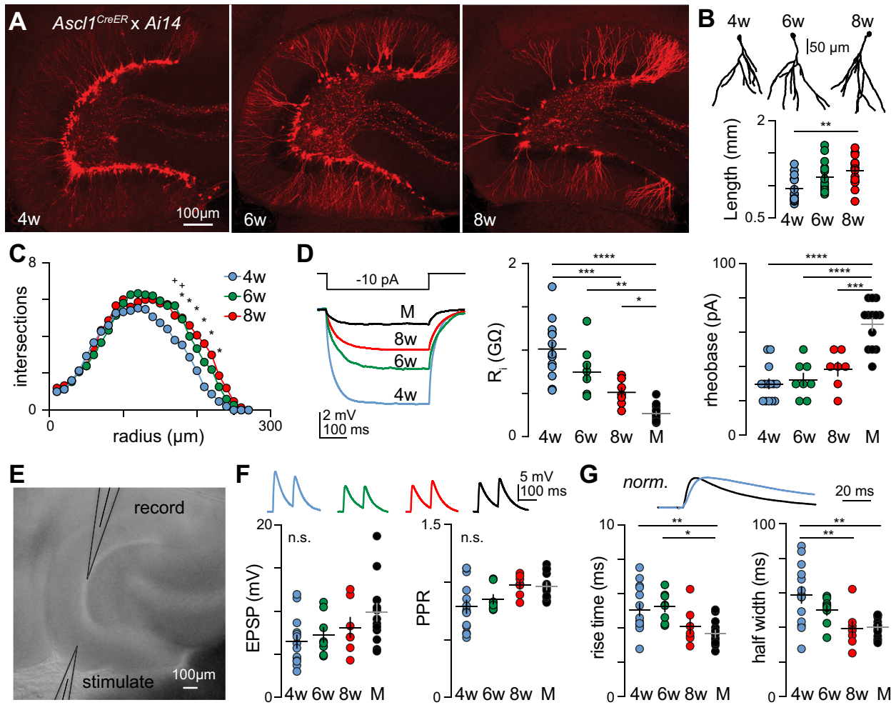
Figure 1. Properties of abGCs. A , Confocal images of abGCs from fixed slices (50 \mu m thick). B , Example reconstructions and TDLs ( n = 15 cells from 2 mice each). One-way ANOVA, F_{(2,42)} = 5.80 , p = 0.006 ; Tukey's post hoc test 4w versus 8w p = 0.005 . C , Sholl analysis. Two-way ANOVA main effect of cell age, F_{(2,42)} = 4.2 , p = 0.02 ; main effect of radius, F_{(26, 1,092)} = 91 , p < 0.0001 ; interaction effect, F_{(52, 1,092)} = 1.54 , p = 0.009 ; Tukey's post hoc test; +, 4w versus 6w p < 0.05 ; *, 4w versus 8w p < 0.05 . D , Left, Examples of hyperpolarization induced by -10 pA current steps. Middle, input resistance ( R_i ) decreased with cell age. 4w, n = 14 ; 6w, n = 8 ; 8w, n = 7 ; M, n = 13 ; Welch's ANOVA, F_{(3,0,15,5)} = 27 , p < 0.0001 ; Dunnett's T3 multiple comparisons with 4w versus M p < 0.0001 , 4w versus 8w p = 0.0007 , 6w versus M p = 0.01 , 8w versus M p = 0.02 . Right, rheobase was lower in abGCs compared to mature GCs, one-way ANOVA, F_{(3,38)} = 24 , p < 0.0001 ; Dunnett's T3 multiple comparisons, p > 0.05 . E , Live image showing typical recording configuration. F , EPSPs had similar amplitude (Kruskal–Wallis test; H_{(3)} = 7.0 , p = 0.07 ) and PPR (Welch's ANOVA; W_{(3,0,19)} = 4.1 , p = 0.02 ; Dunnett's multiple comparisons, p > 0.05 ). G , Normalized EPSPs highlighting different rise and decay kinetics. Rise: one-way ANOVA; F_{(3,38)} = 5.5 , p = 0.003 ; Dunnett's T3 multiple comparisons, 4w versus M p = 0.008 , 6w versus M p = 0.01 . Half-width: one-way ANOVA F_{(3,38)} = 6.7 , p = 0.001 ; Tukey's post hoc tests, 4w versus M p = 0.002 , 4w versus 8w p = 0.008 . n.s., not significant, * p < 0.05 , ** p < 0.01 , *** p < 0.001 , **** p < 0.0001 . All error bars \pm SEM.
