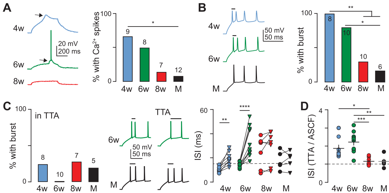
Figure 4. Sensitivity to T-type \text{Ca}^{2+} channel antagonist correlates with the critical period. A , Examples of putative T-type \text{Ca}^{2+} spikelets (arrows) in 4w and 6w abGCs from perforated patch recordings. The spikelet reaches threshold for a \text{Na}^+ action potential in the 6w abGC. Multiple Fisher's exact tests, 4w versus M p = 0.02 . Total number of cells as indicated. B , Typical firing patterns in whole-cell recordings, with action potential bursts indicated by lines. Multiple Fisher's exact tests, 4w versus 8w and M p = 0.003 , 6w versus M p = 0.04 . C , Left, Percent of cells in TTA with bursts. Multiple Fisher's exact tests, not significant. Middle, Example firing patterns with first spike ISIs indicated in control (left) and TTA (right). Right, ISI in ACSF (circles) and TTA (triangles). Dotted line indicates ISI of 15 ms. Two-way RM ANOVA main effect cell age, F_{(3,26)} = 3.0 , p = 0.048 ; main effect TTA, F_{(1,26)} = 27 , p < 0.0001 ; interaction effect, F_{(3,26)} = 9.06 , p = 0.0003 ; Bonferroni's multiple comparisons, 4w p = 0.004 , 6w p < 0.0001 . D , The ISI in TTA relative to the ISI in ACSF (dotted line). One-way ANOVA F_{(3,26)} = 9.2 , p = 0.0002 ; Tukey's post hoc comparison, 4w versus 8w p = 0.04 , 6w versus 8w p = 0.0008 , 6w versus M p = 0.002 . 4w, n = 8 ; 6w, n = 10 ; 8w, n = 7 ; M, n = 5 .
